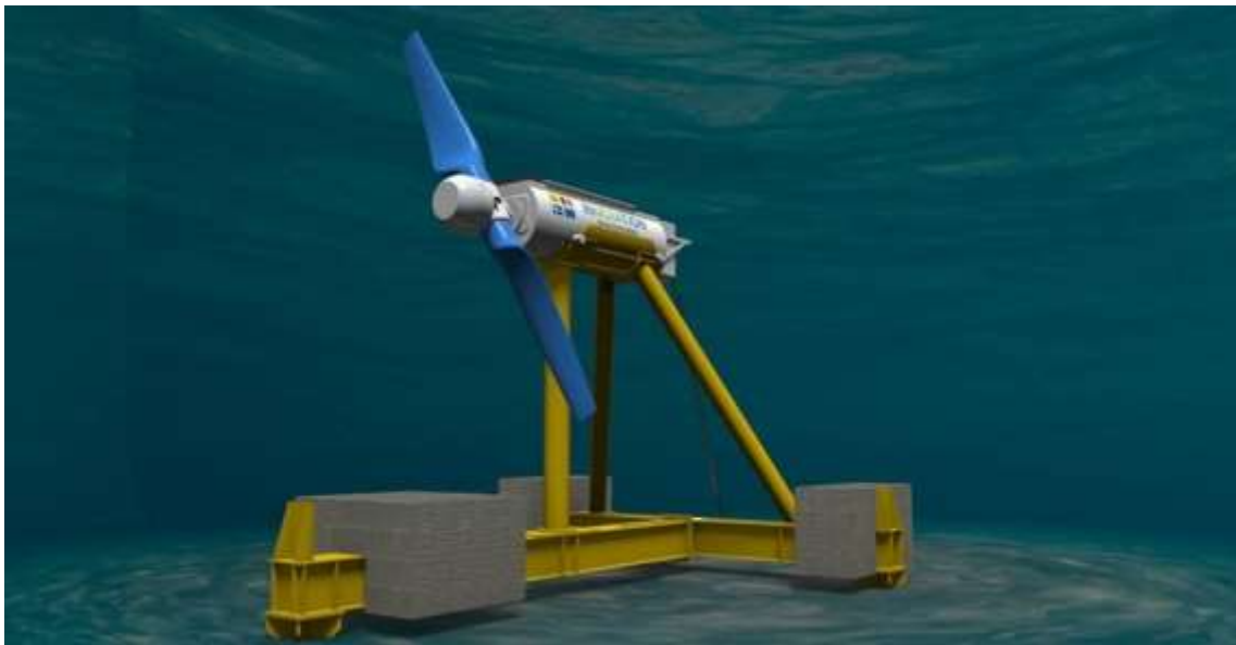
Figure 1. Nova Innovation Tidal Device
